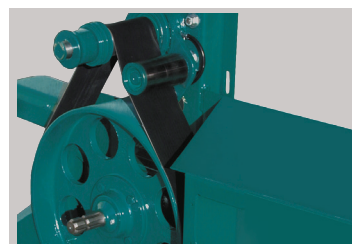
Power band fan speed up system with built-in overrunning clutch
