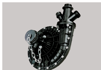
Low pressure centrifugal pump made of anti-corrosive material requires little maintenance
