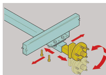
Wheels adjust up or down, in or out, front or rear to obtain best balance and clearance
